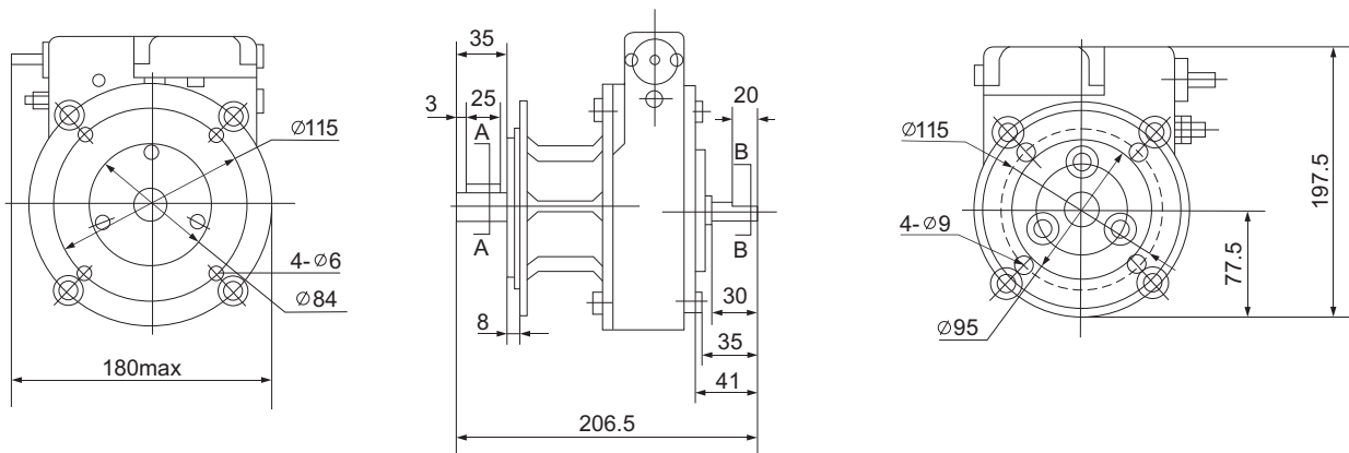
LLY1-1X/□D型超速开关外形及安装尺寸 LLY1-1X/□D overspeed switch Shape and mounting dimensions
