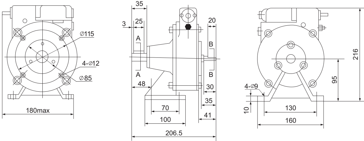
LLY1-1X/□型超速开关外形及安装尺寸 LLY1-1X/□ overspeed switch Shape and mounting dimensions
